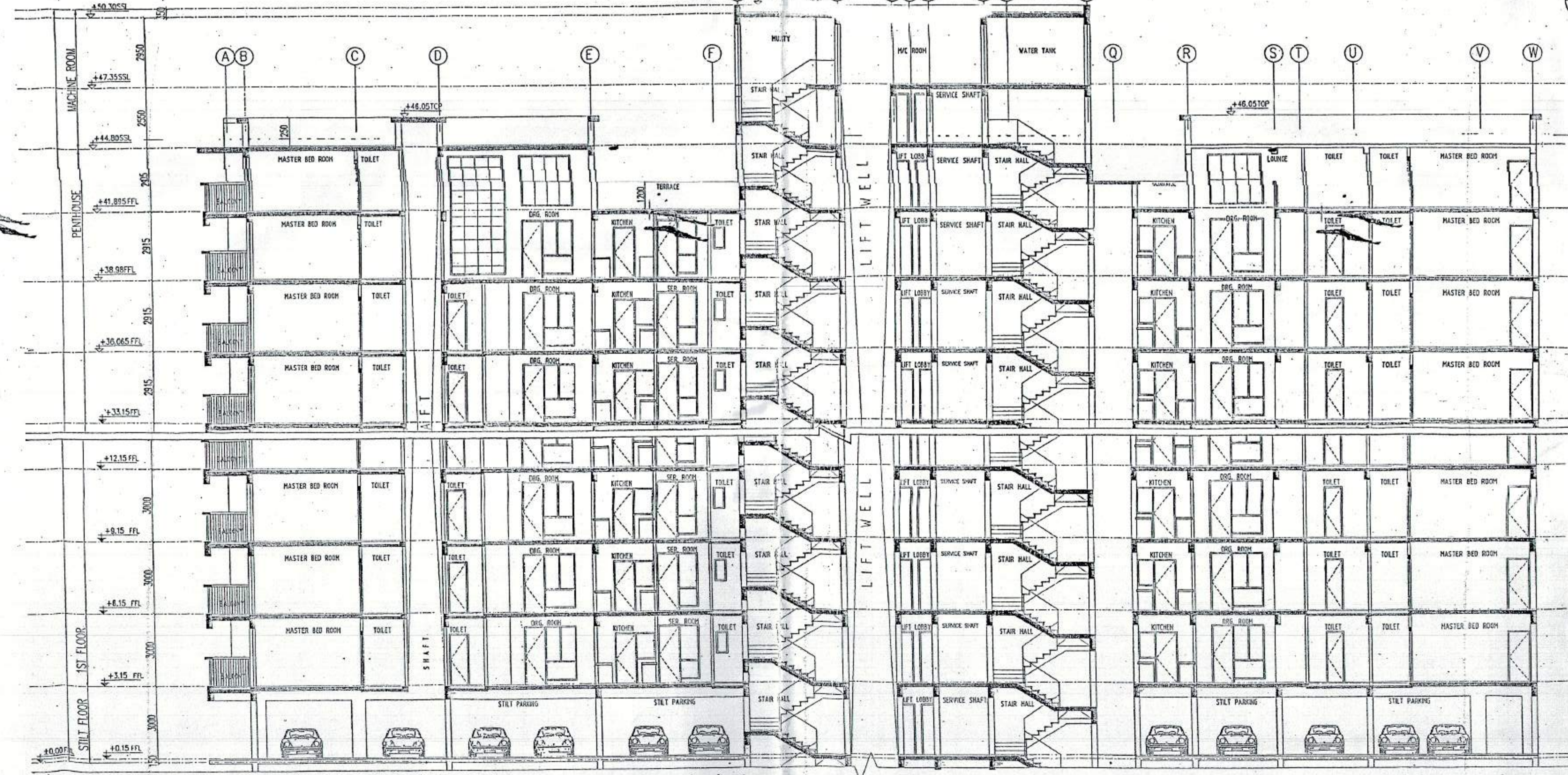
A SECTION - S1 (SCALE 1:100)
