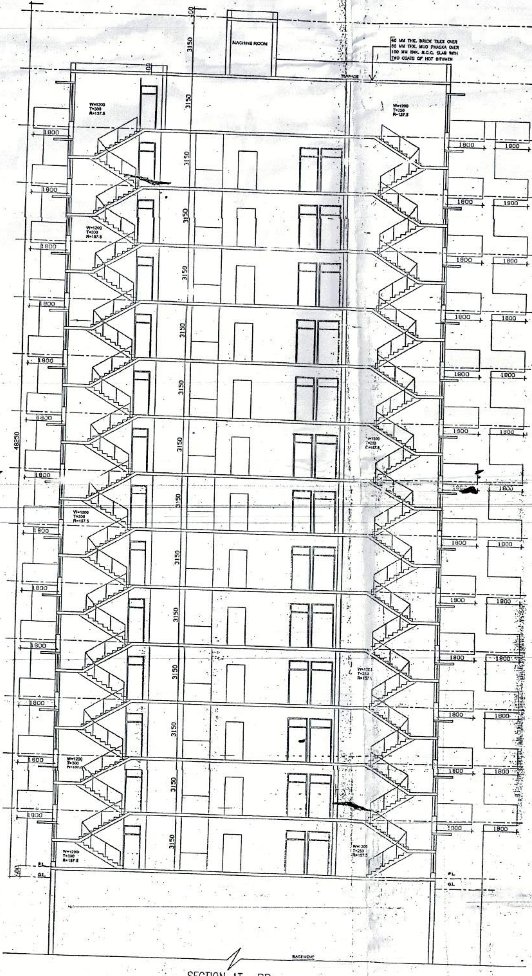
SECTION AT -BB
